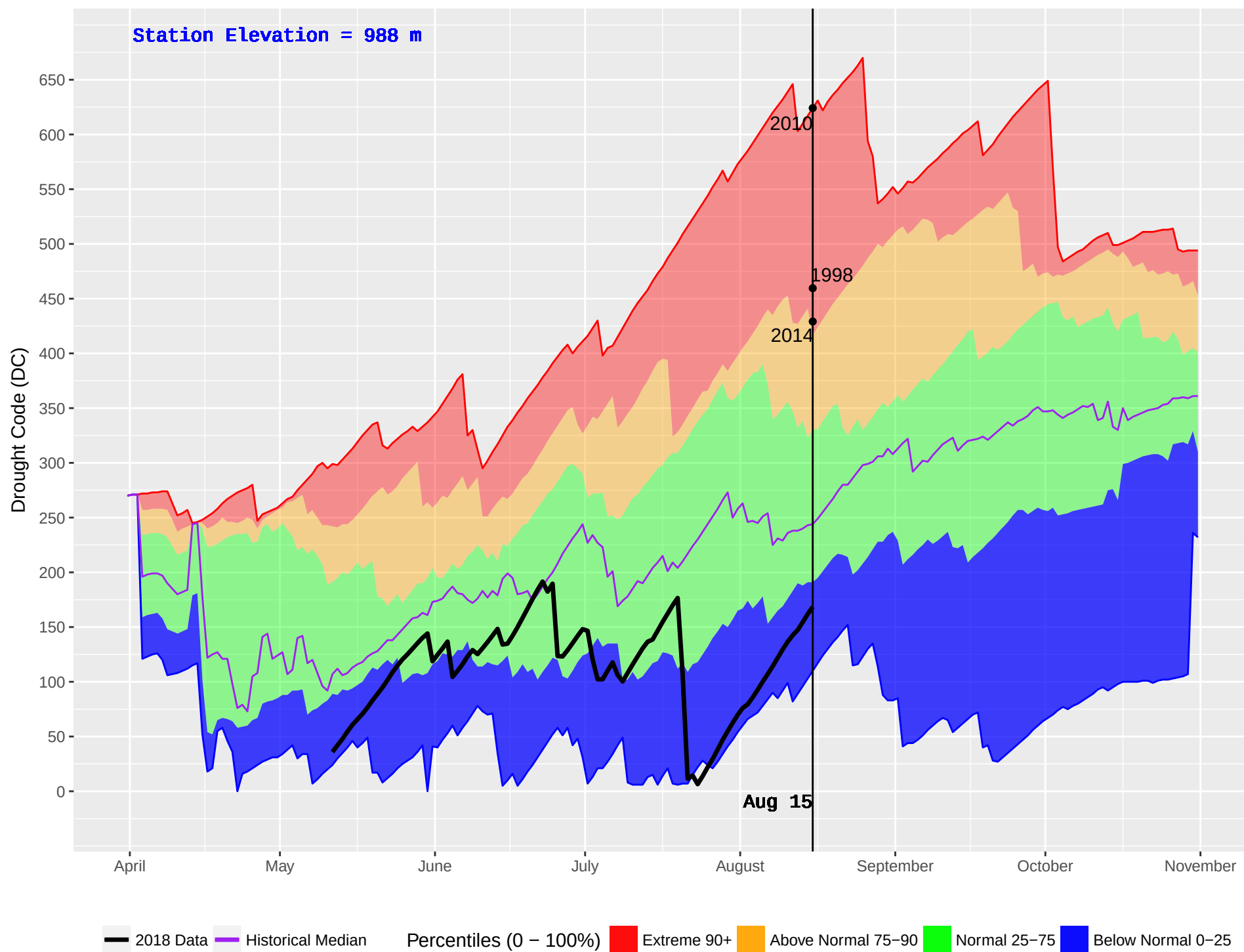
NOEL (437) : Historical (1993–2016) and Current (2018) Daily Drought Code (DC)
