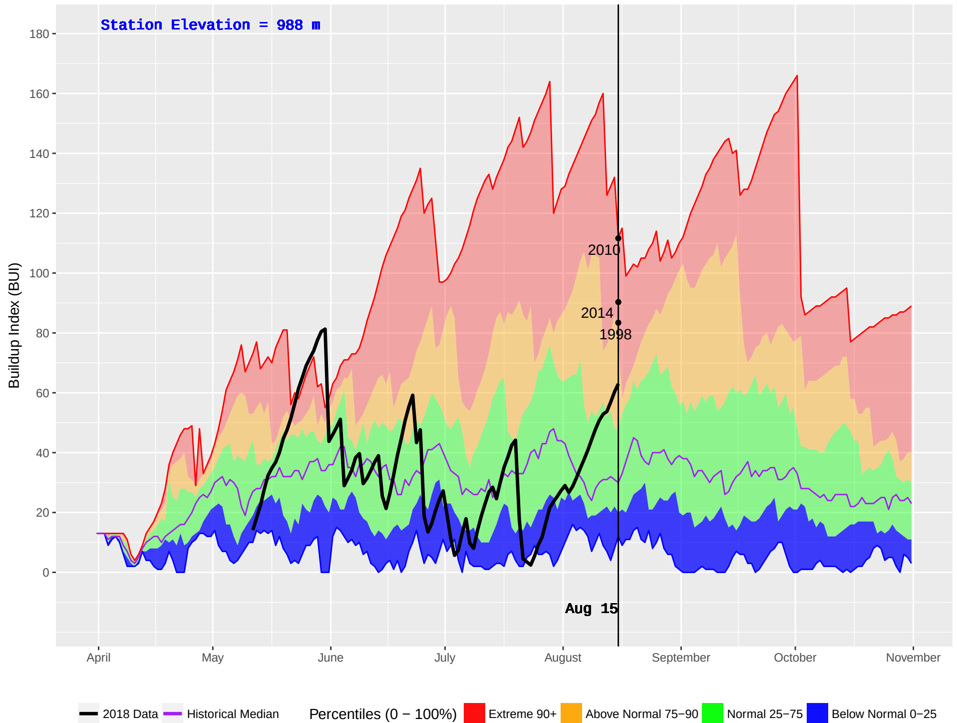
NOEL (437) : Historical (1993–2016) and Current (2018) Daily Buildup Index (BUI)
