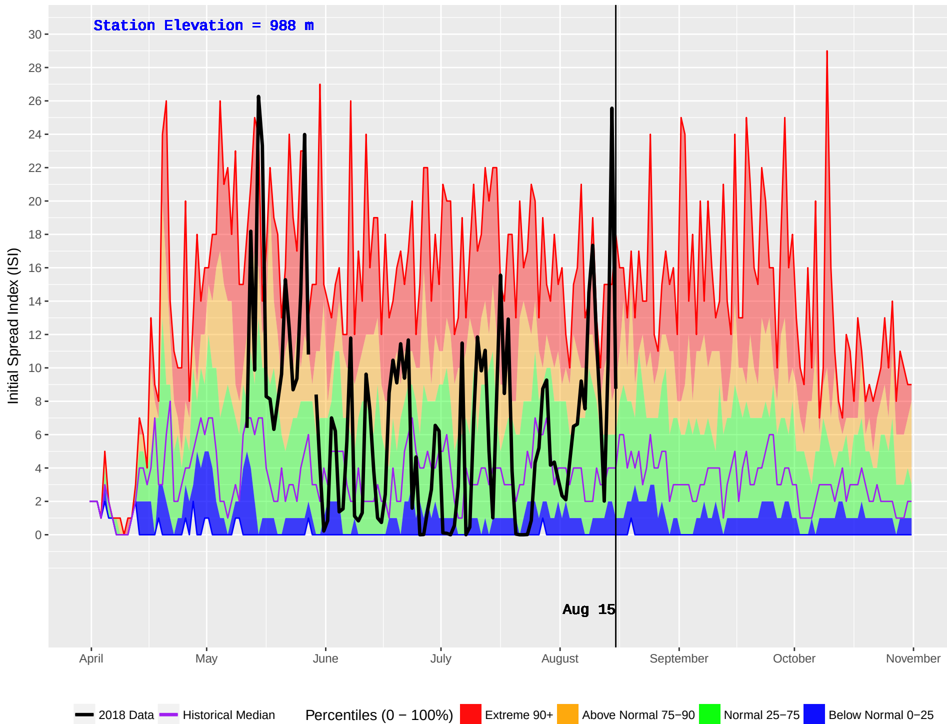
NOEL (437) : Historical (1993–2016) and Current (2018) Daily Initial Spread Index (ISI)
