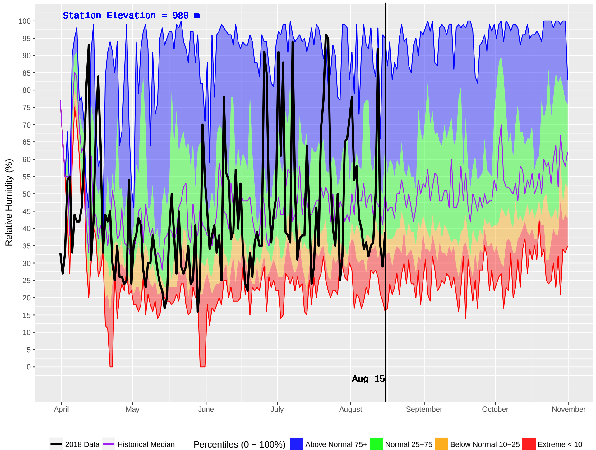
NOEL (437) : Historical (1993–2016) and Current (2018) Daily Relative Humidity
