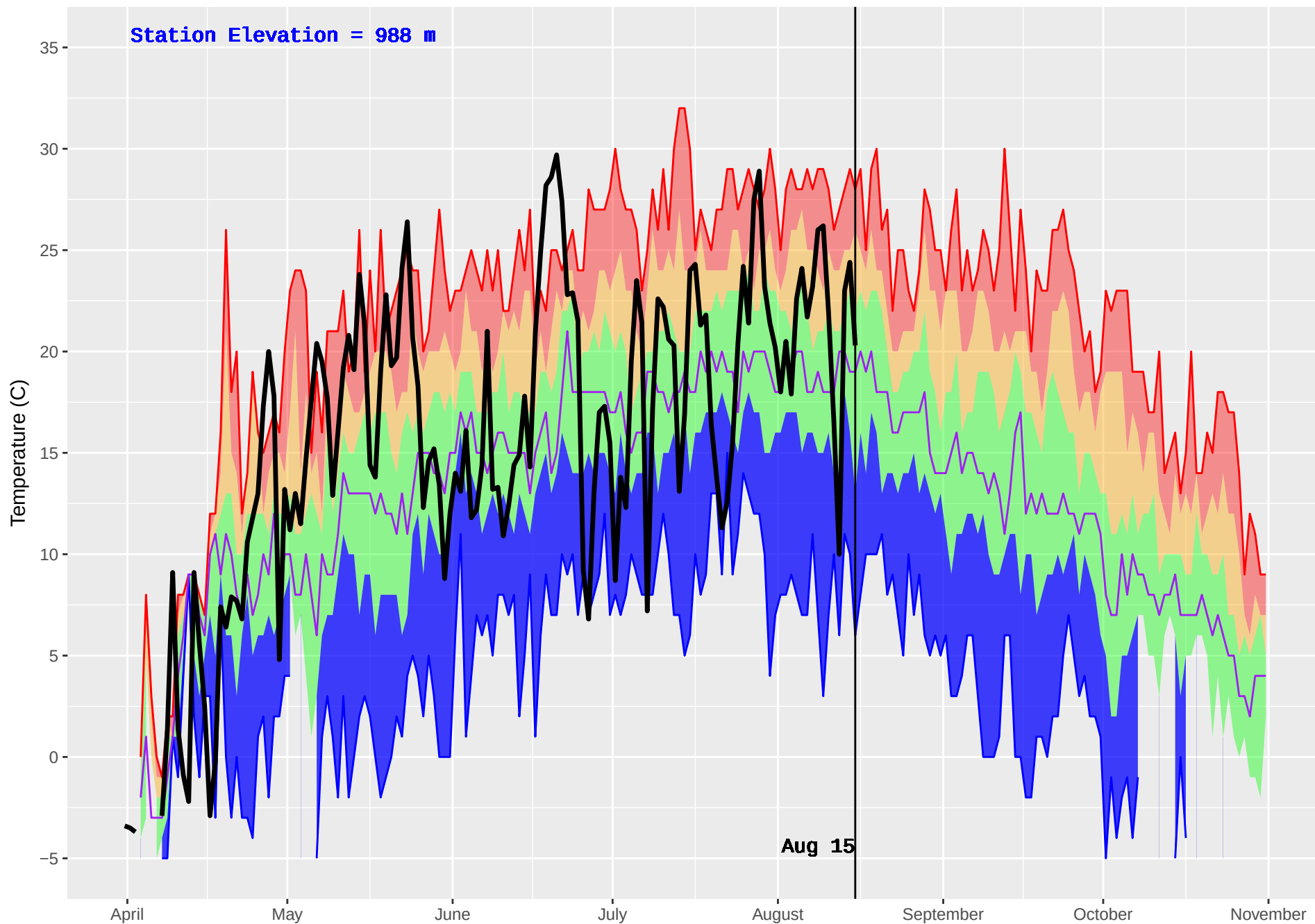
NOEL (437) : Historical (1993–2016) and Current (2018) Daily Temperature
