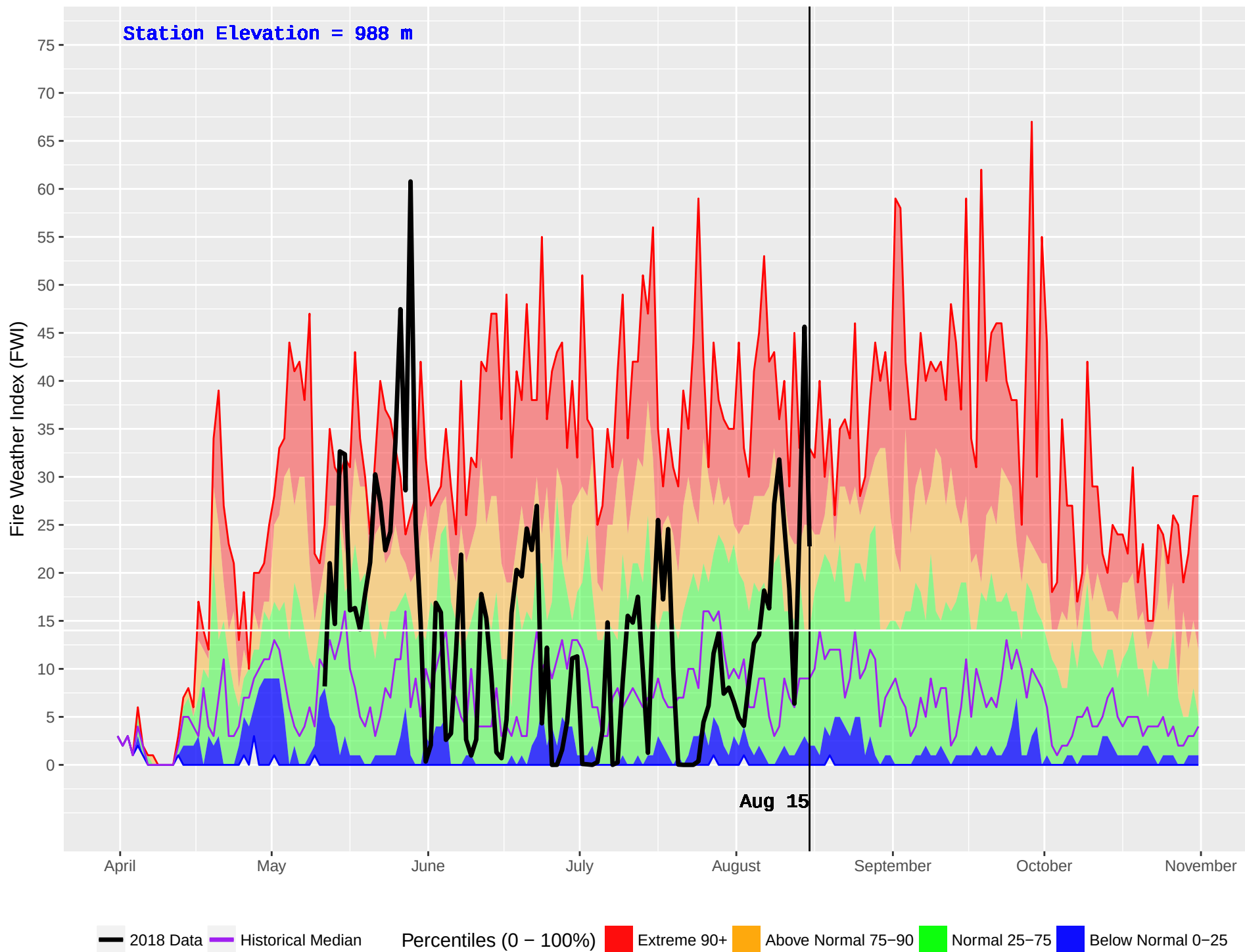
NOEL (437) : Historical (1993–2016) and Current (2018) Daily Fire Weather Index (FWI)
